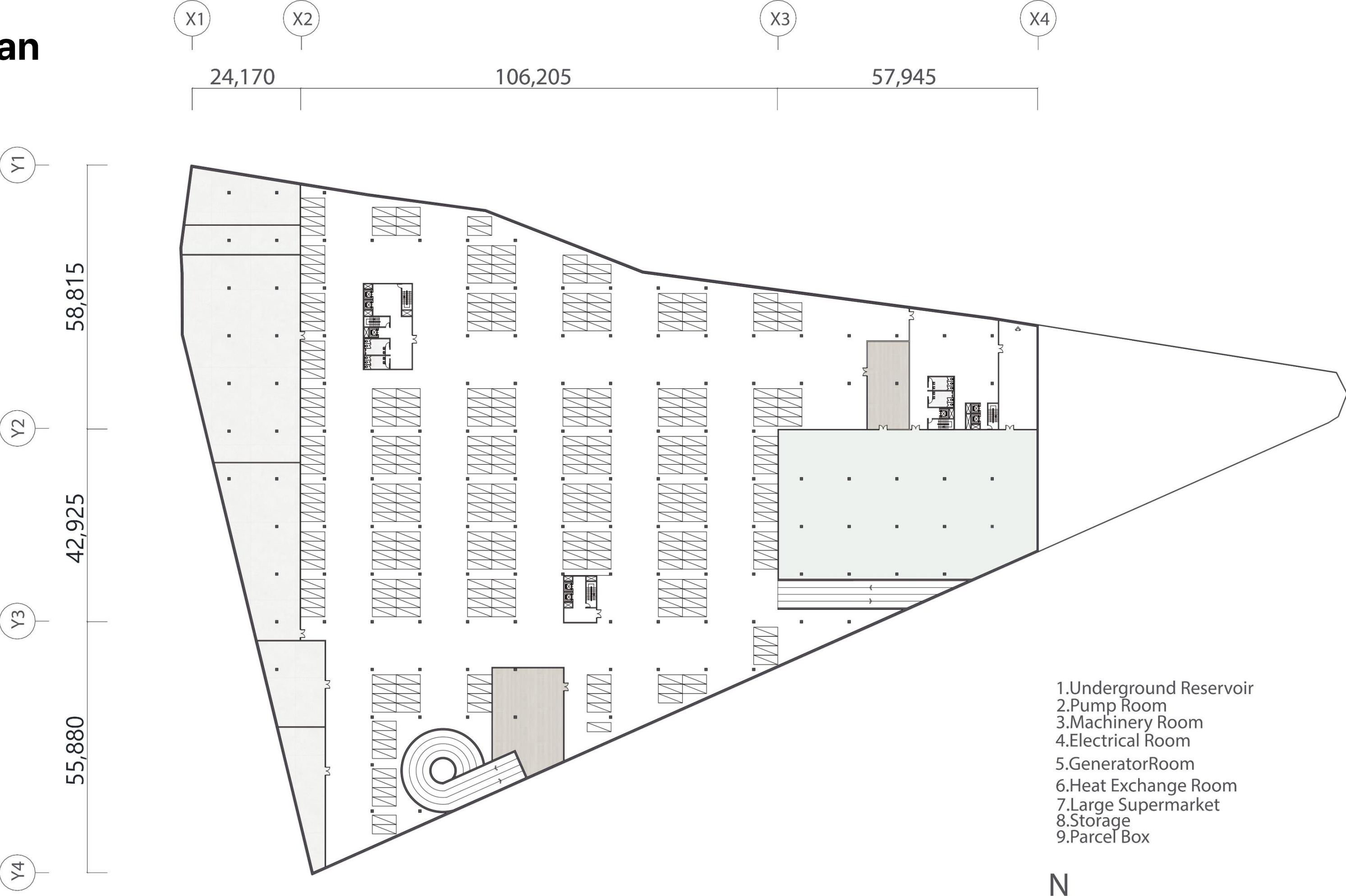
B1F FLOOR PLAN SCALE 1/1000
